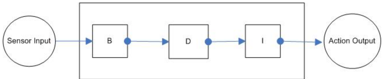
Figure 2. BDI architecture
