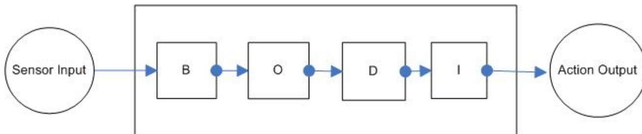
Figure 3. BOID architecture
