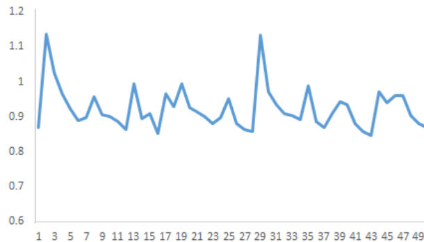
Figure 7: Plot of simulated loss ratio over time (years) for one simulation run of the agent-based model of the UK property insurance sector.
