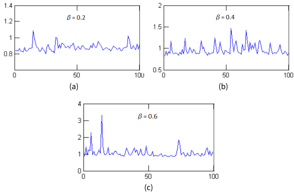
Figure 9: Time plots of simulated loss ratio for \beta = 0.2 (top panel), \beta = 0.4 (middle panel), \beta = 0.6 (bottom panel). The loss ratio becomes more volatile as \beta increases. (The vertical scales in the 3 panels are different.)
