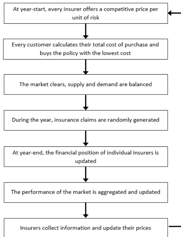
Figure 4: An outline of the insurance agent-based model.
